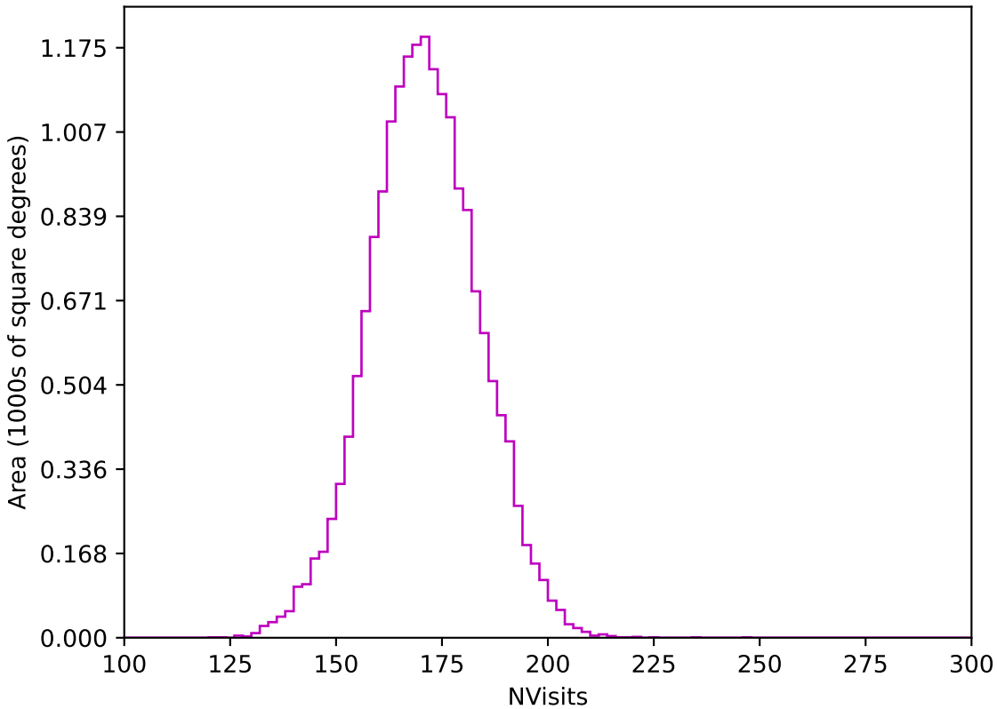
ddf_acor_sf30_lsf40_lsr20_v3.4_10yrs WFD z band: NVisits
