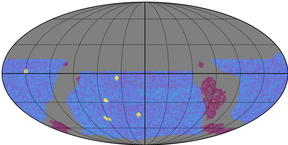
ddf_acor_sf30_lsf40_lsr20_v3.4_10yrs WFD y band: NVisits
