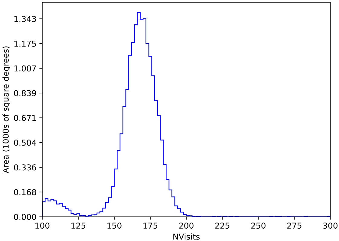
ddf_acor_sf30_lsf40_lsr20_v3.4_10yrs WFD y band: NVisits
