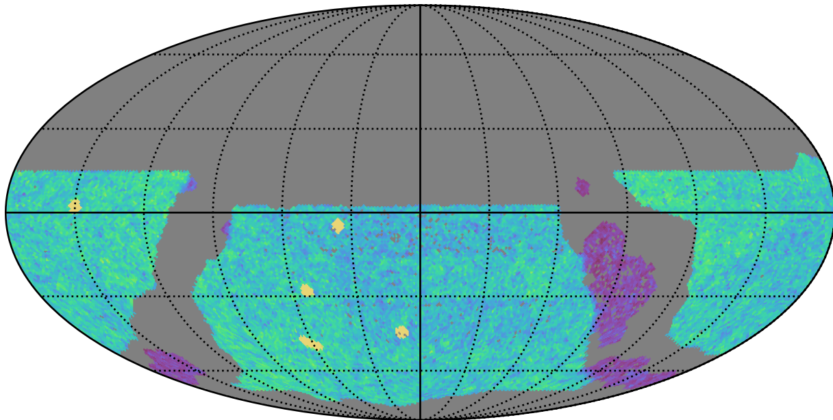
ddf_acor_sf30_lsf40_lsr20_v3.4_10yrs WFD u band: NVisits
