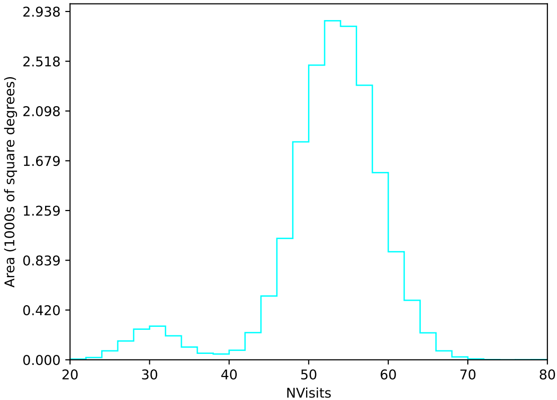
ddf_acor_sf30_lsf40_lsr20_v3.4_10yrs WFD u band: NVisits
