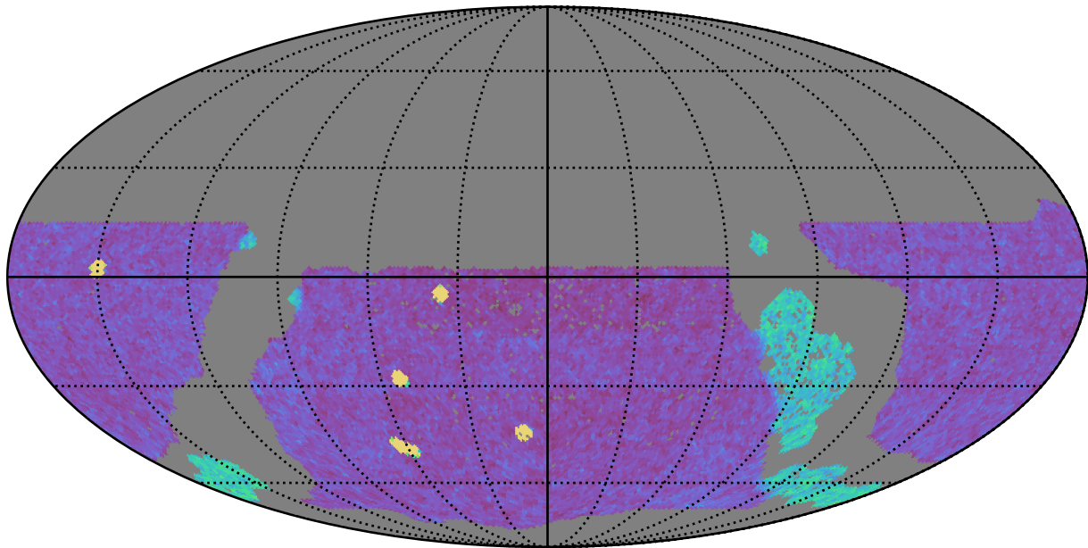
ddf_acor_sf30_lsf40_lsr20_v3.4_10yrs WFD g band: NVisits
