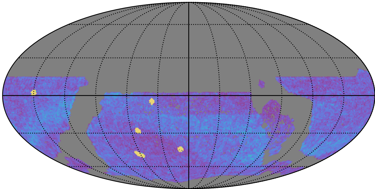
ddf_acor_sf30_lsf40_lsr20_v3.4_10yrs WFD all bands: NVisits
