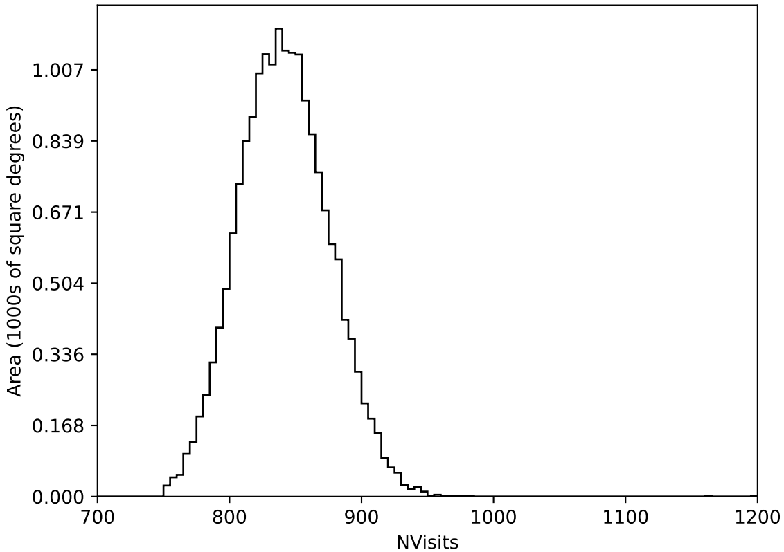
ddf_acor_sf30_lsf40_lsr20_v3.4_10yrs WFD all bands: NVisits
