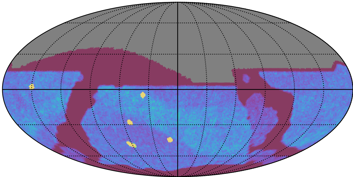
ddf_acor_sf30_lsf40_lsr20_v3.4_10yrs All sky z band: NVisits
