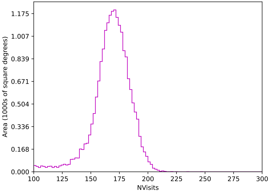
ddf_acor_sf30_ls40_lsr20_v3.4_10yrs All sky z band: NVisits
