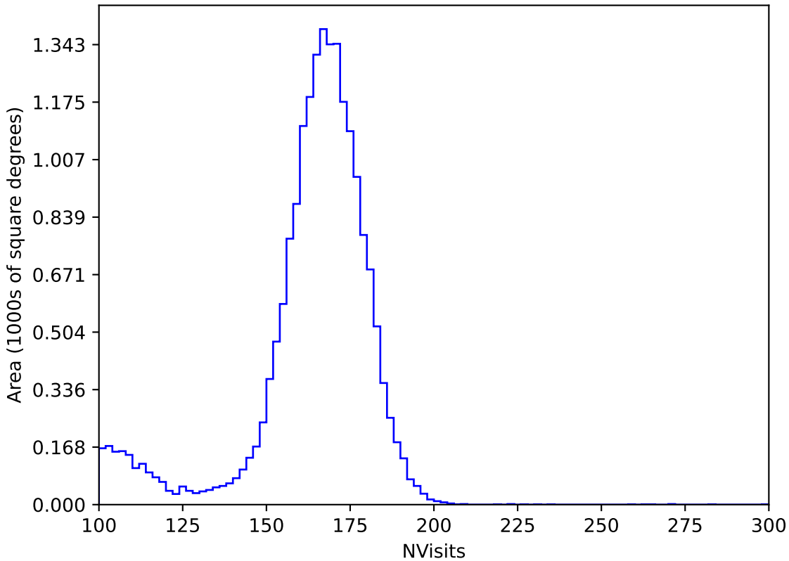
ddf_acor_sf30_lsf40_lsr20_v3.4_10yrs All sky y band: NVisits
