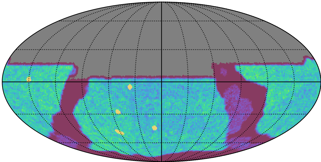
ddf_acor_sf30_lsf40_lsr20_v3.4_10yrs All sky u band: NVisits
