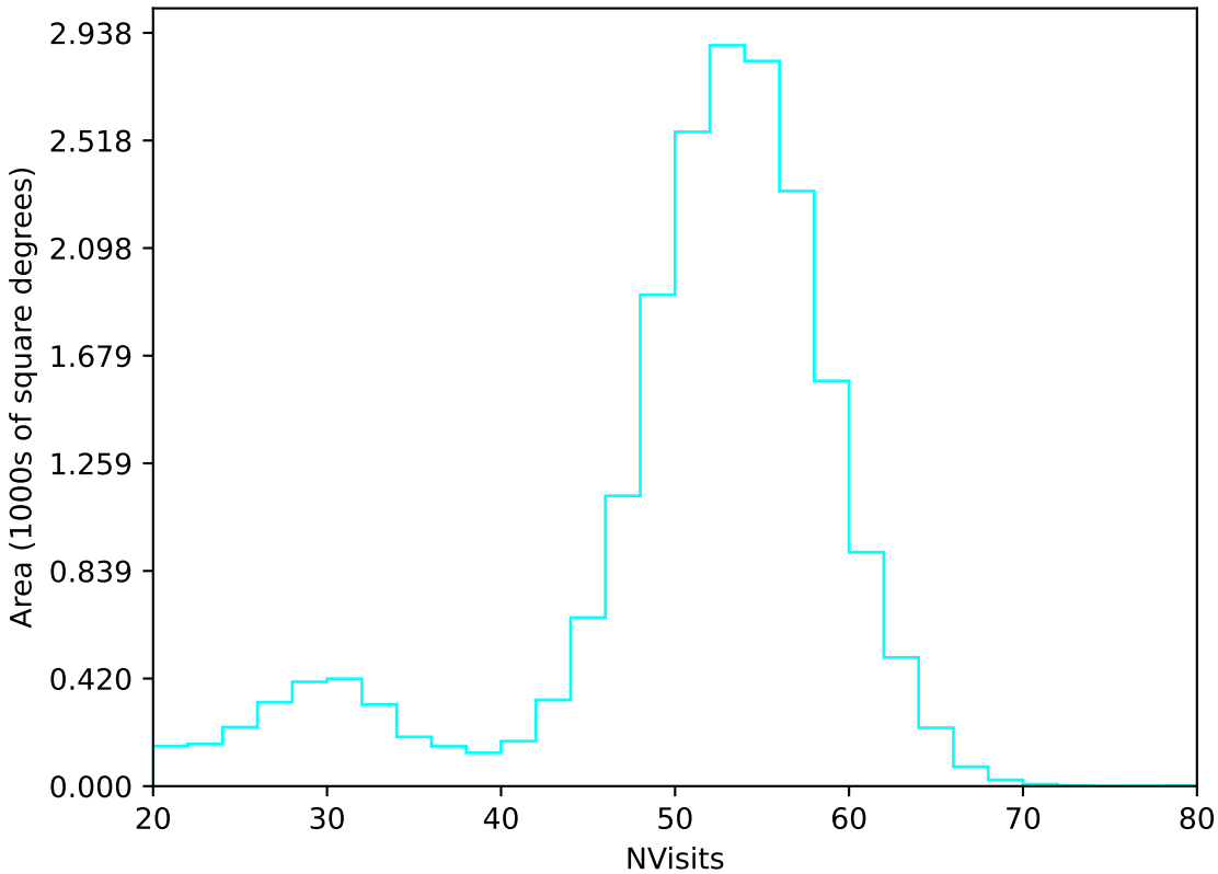
ddf_acor_sf30_lsf40_lsr20_v3.4_10yrs All sky u band: NVisits
