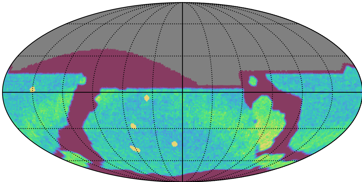
ddf_acor_sf30_lsf40_lsr20_v3.4_10yrs All sky r band: NVisits
