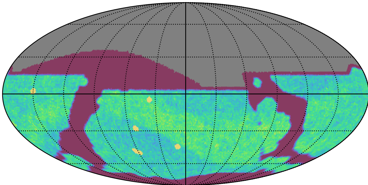
ddf_acor_sf30_lsf40_lsr20_v3.4_10yrs All sky i band: NVisits
