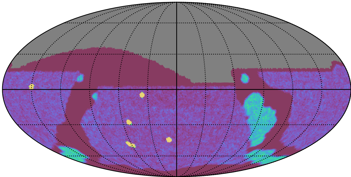
ddf_acor_sf30_lsf40_lsr20_v3.4_10yrs All sky g band: NVisits
