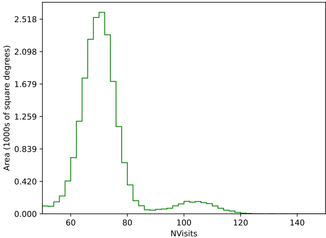
ddf_acor_sf30_lsf40_lsr20_v3.4_10yrs All sky g band: NVisits
