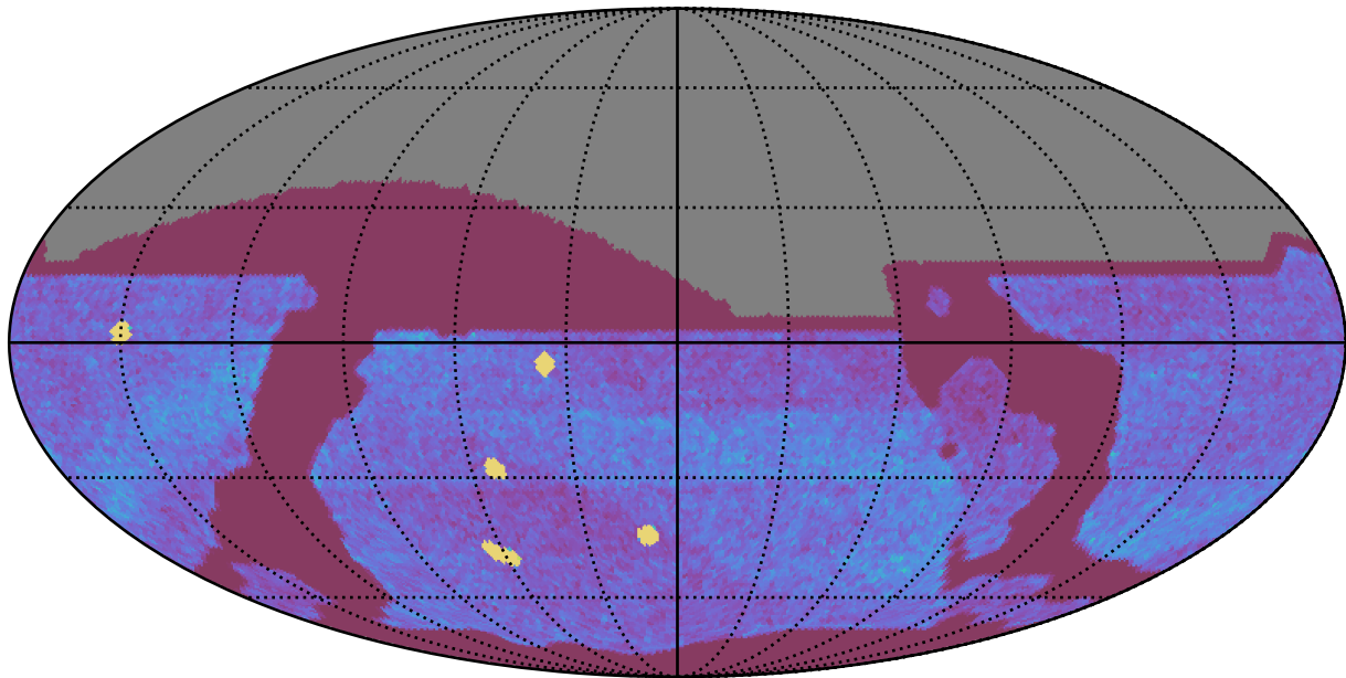
ddf_acor_sf30_lsf40_lsr20_v3.4_10yrs All sky all bands: NVisits
