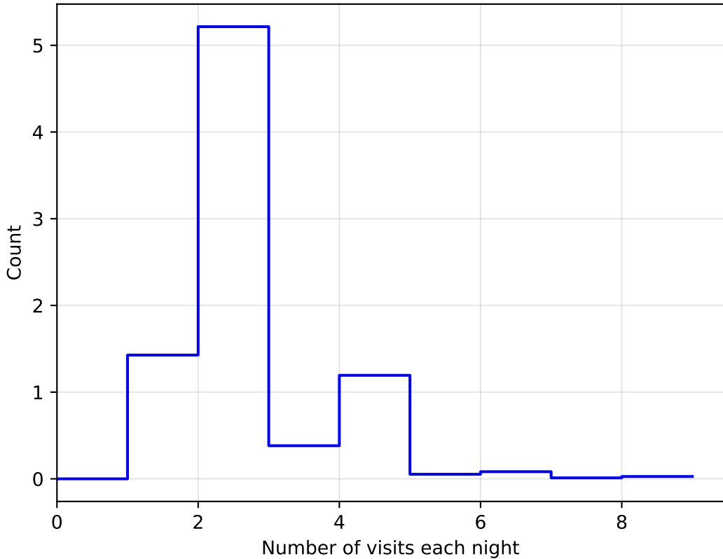
ddf_acor_sf30_lsf40_lsr20_v3.4_10yrs WFD: NVisitsPerNight 1e6
