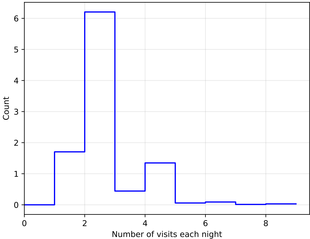
ddf_acor_sf30_lsf40_lsr20_v3.4_10yrs All sky: NVisitsPerNight 1e6
