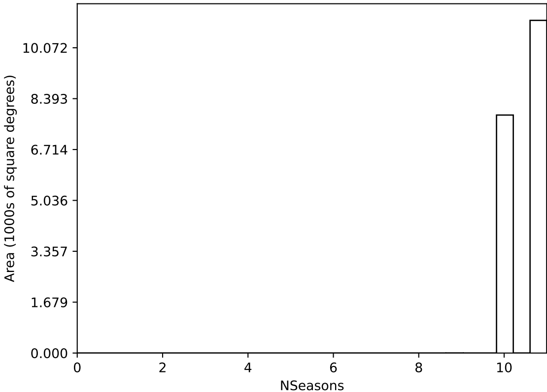
ddf_acor_sf30_lsf40_lsr20_v3.4_10yrs WFD all bands: NSeasons
