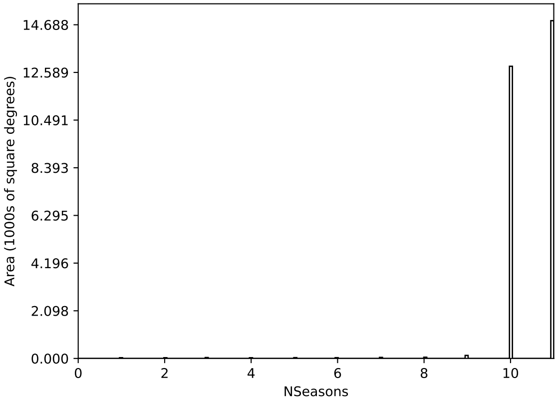
ddf_acor_sf30_lsf40_lsr20_v3.4_10yrs All sky all bands: NSeasons
