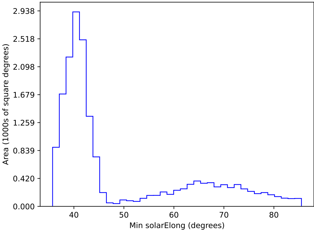
ddf_acor_sf30_lsf40_lsr20_v3.4_10yrs WFD z band: Min solarElong
