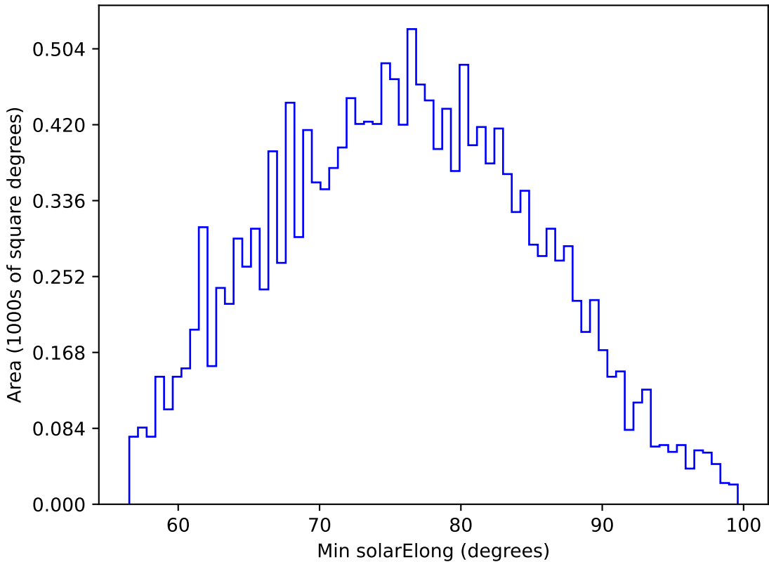
ddf_acor_sf30_lsf40_lsr20_v3.4_10yrs WFD u band: Min solarElong
