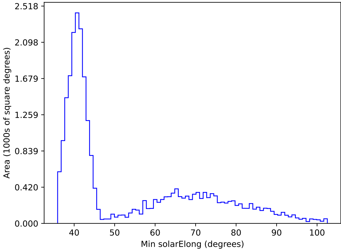
ddf_acor_sf30_lsf40_lsr20_v3.4_10yrs All sky z band: Min solarElong
