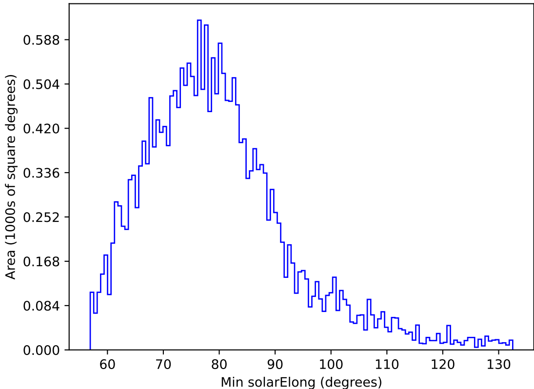
ddf_acor_sf30_lsf40_lsr20_v3.4_10yrs All sky u band: Min solarElong
