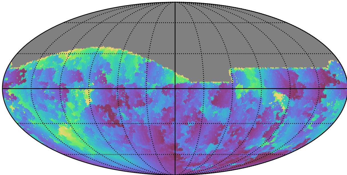
ddf_acor_sf30_lsf40_lsr20_v3.4_10yrs All sky g band: Min solarElong
