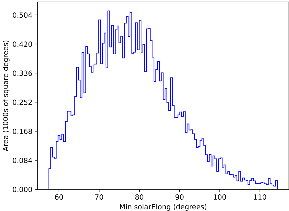
ddf_acor_sf30_lsf40_lsr20_v3.4_10yrs All sky g band: Min solarElong
