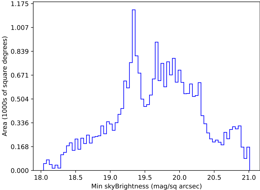
ddf_acor_sf30_lsf40_lsr20_v3.4_10yrs Yr 1 r band: Min skyBrightness
