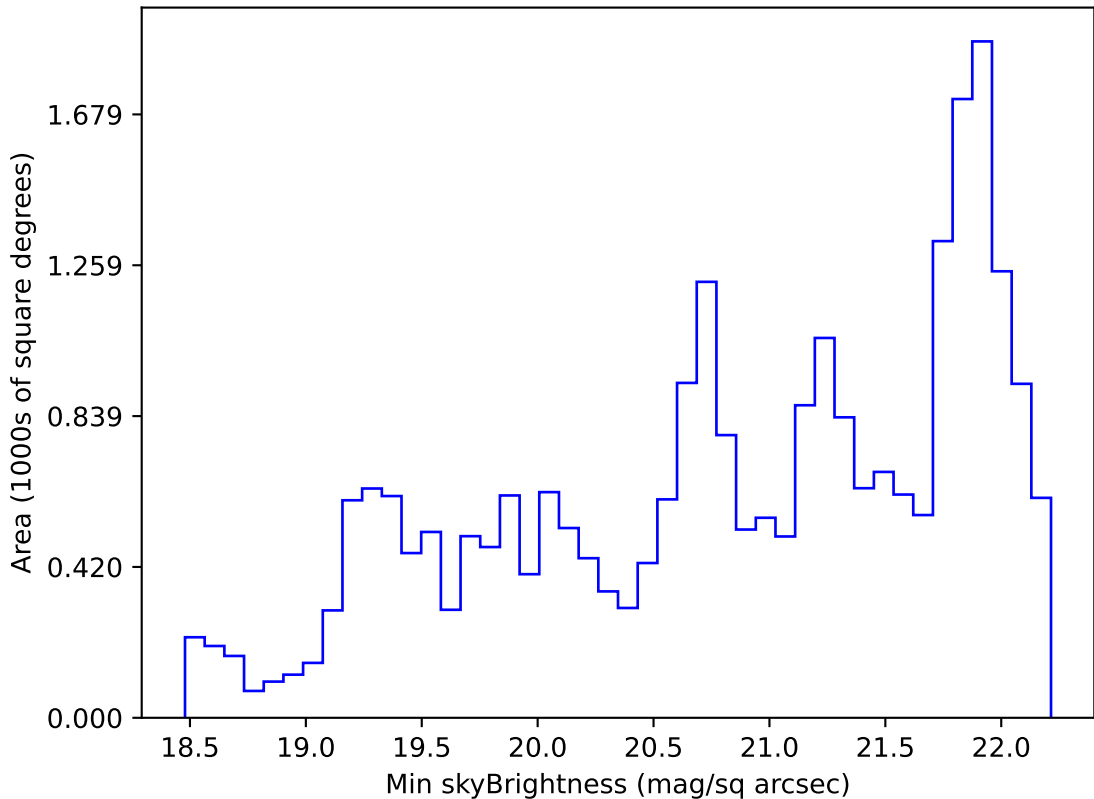
ddf_acor_sf30_lsf40_lsr20_v3.4_10yrs Yr 1 g band: Min skyBrightness
