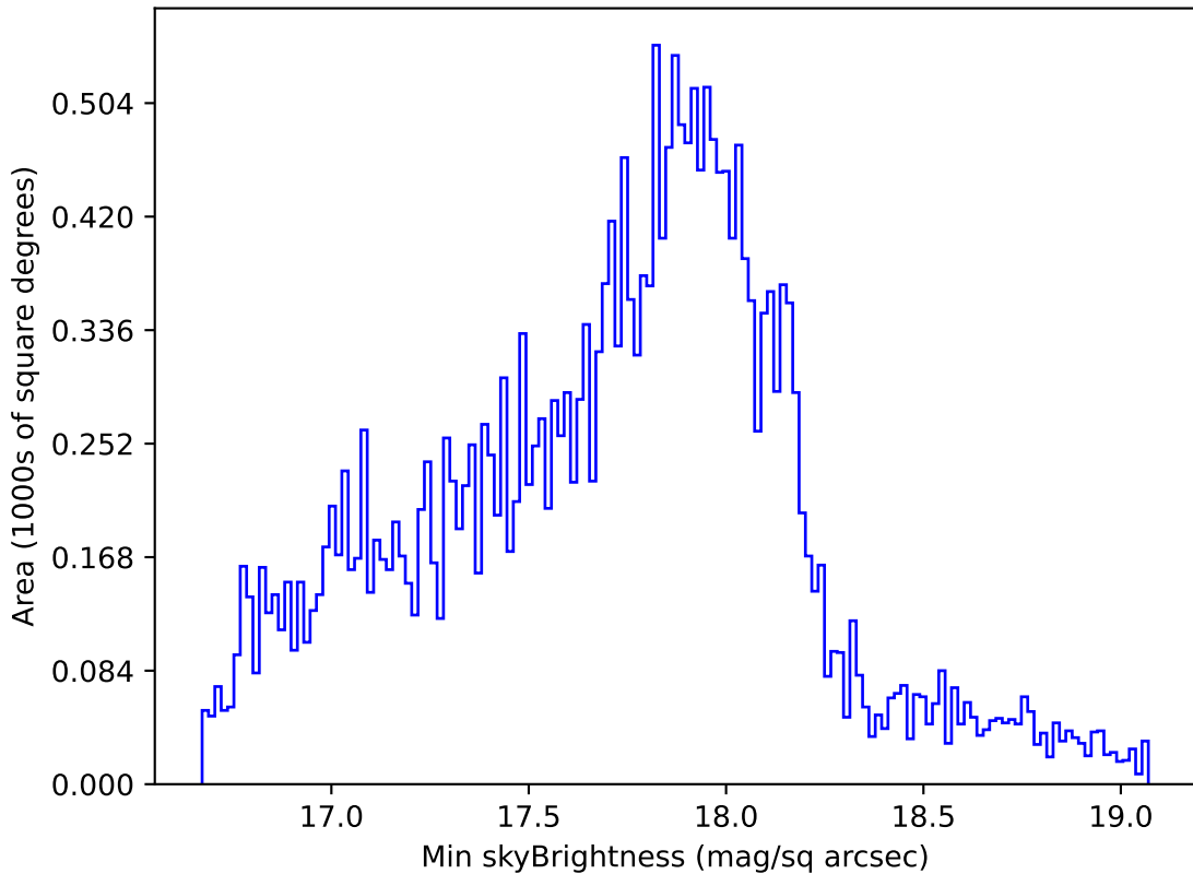
ddf_acor_sf30_lsf40_lsr20_v3.4_10yrs Yr 1 all bands: Min skyBrightness
