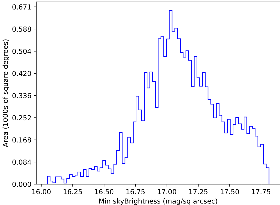
ddf_acor_sf30_lsf40_lsr20_v3.4_10yrs WFD y band: Min skyBrightness
