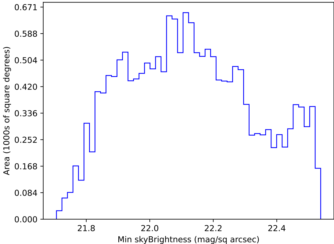
ddf_acor_sf30_lsf40_lsr20_v3.4_10yrs WFD u band: Min skyBrightness
