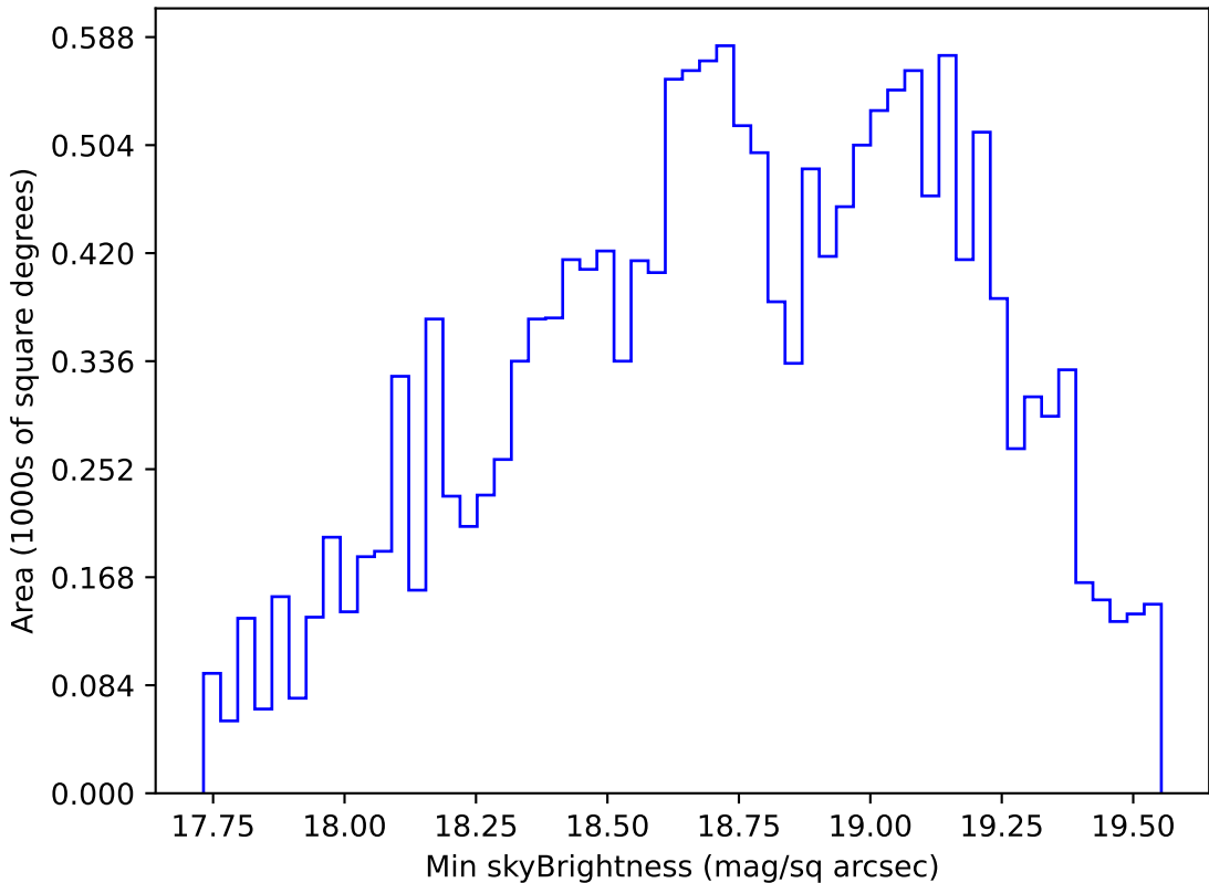
ddf_acor_sf30_lsf40_lsr20_v3.4_10yrs WFD r band: Min skyBrightness
