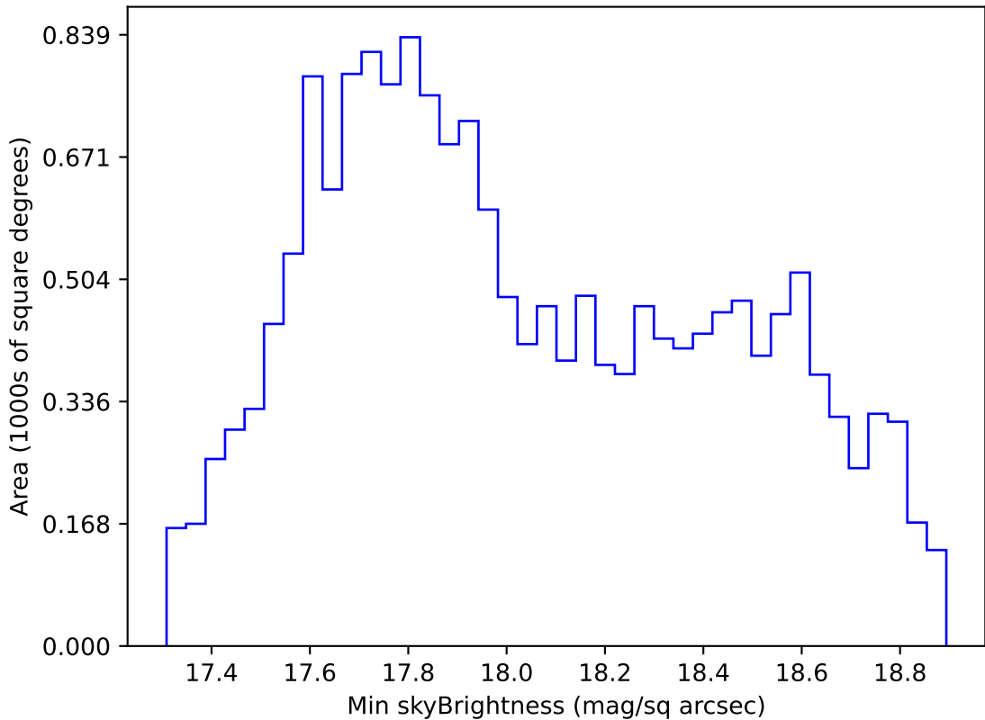
ddf_acor_sf30_lsf40_lsr20_v3.4_10yrs WFD i band: Min skyBrightness
