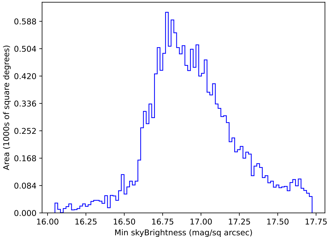
ddf_acor_sf30_lsf40_lsr20_v3.4_10yrs WFD all bands: Min skyBrightness
