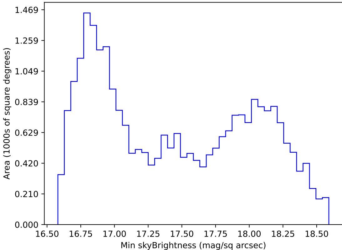
ddf_acor_sf30_lsf40_lsr20_v3.4_10yrs All sky z band: Min skyBrightness
