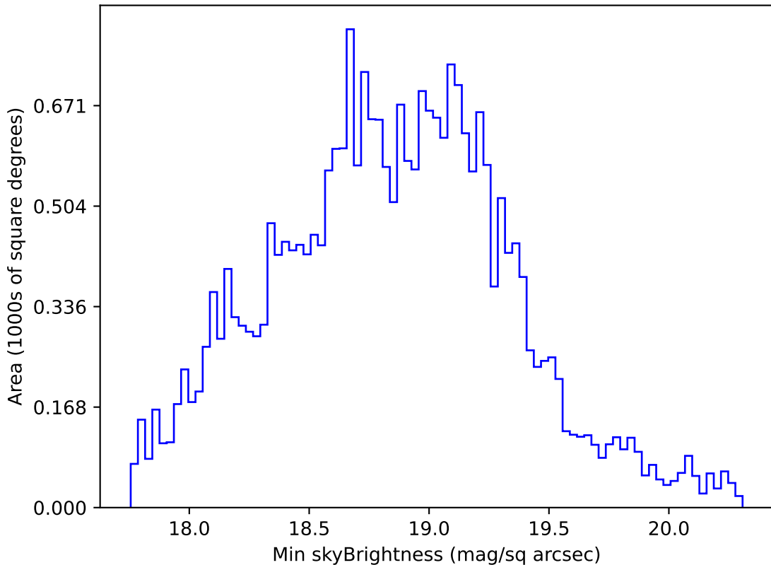
ddf_acor_sf30_lsf40_lsr20_v3.4_10yrs All sky r band: Min skyBrightness
