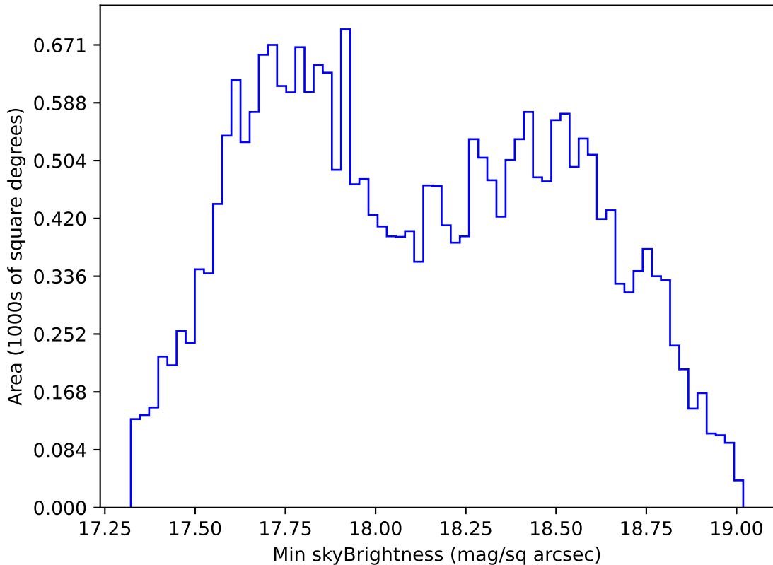
ddf_acor_sf30_lsf40_lsr20_v3.4_10yrs All sky i band: Min skyBrightness
