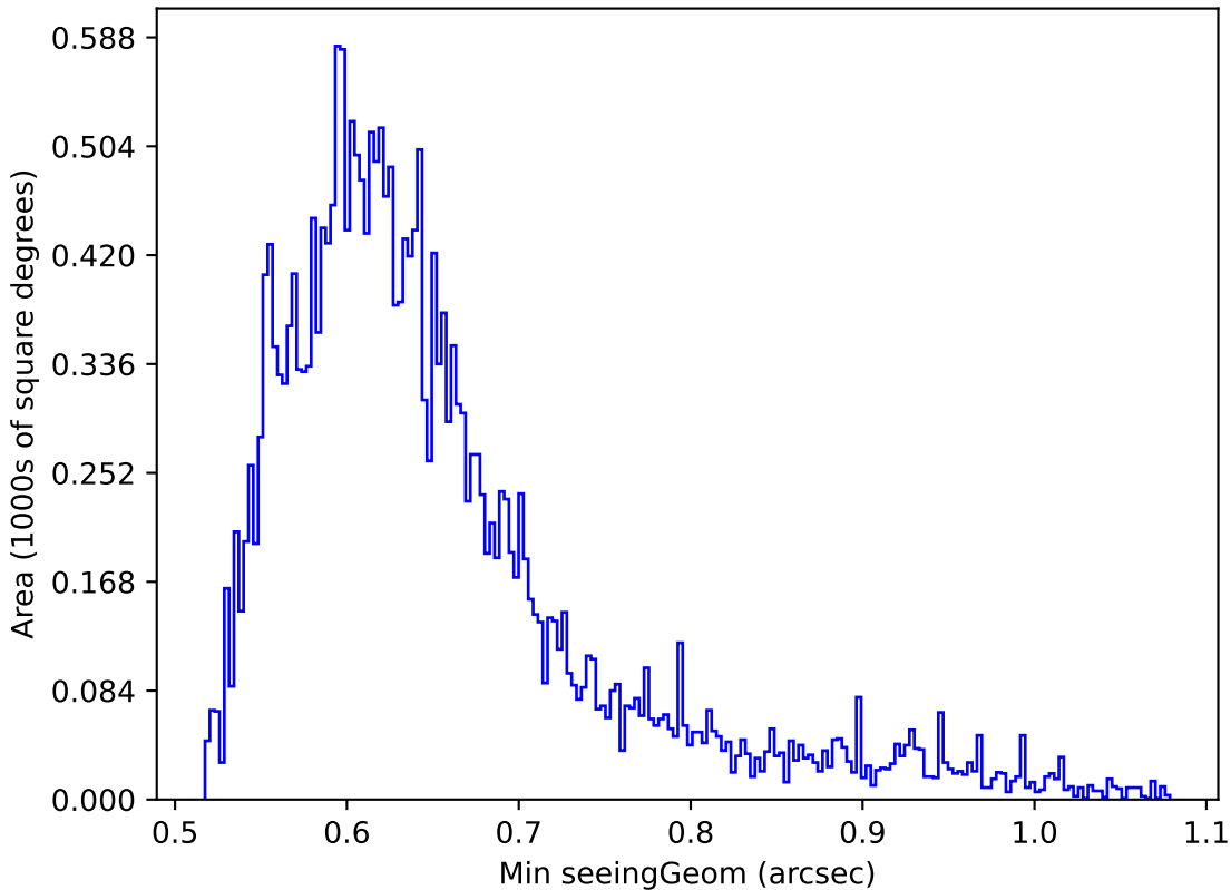
ddf_acor_sf30_lsf40_lsr20_v3.4_10yrs Yr 1 z band: Min seeingGeom
