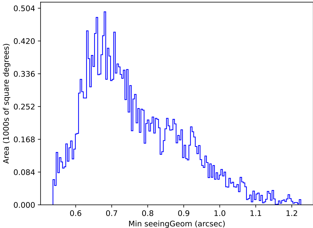
ddf_acor_sf30_lsf40_lsr20_v3.4_10yrs Yr 1 u band: Min seeingGeom
