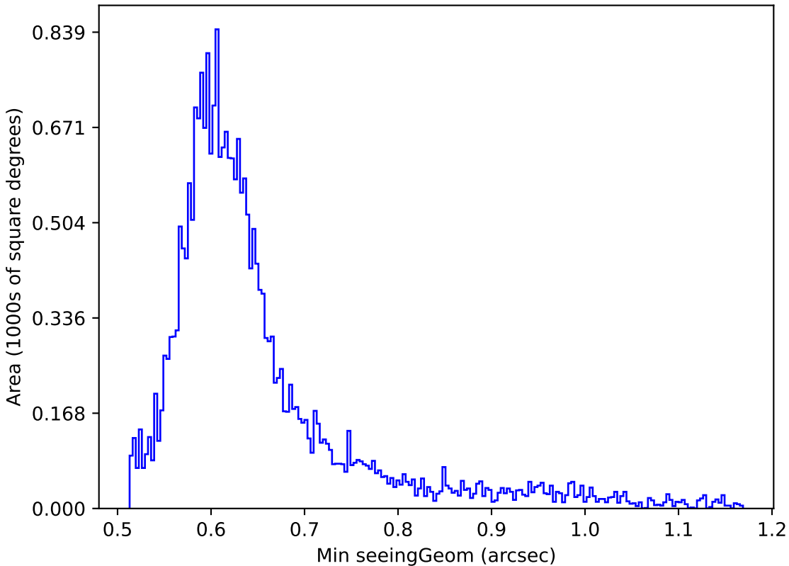
ddf_acor_sf30_Isf40_Isr20_v3.4_10yrs Yr 1 r band: Min seeingGeom
