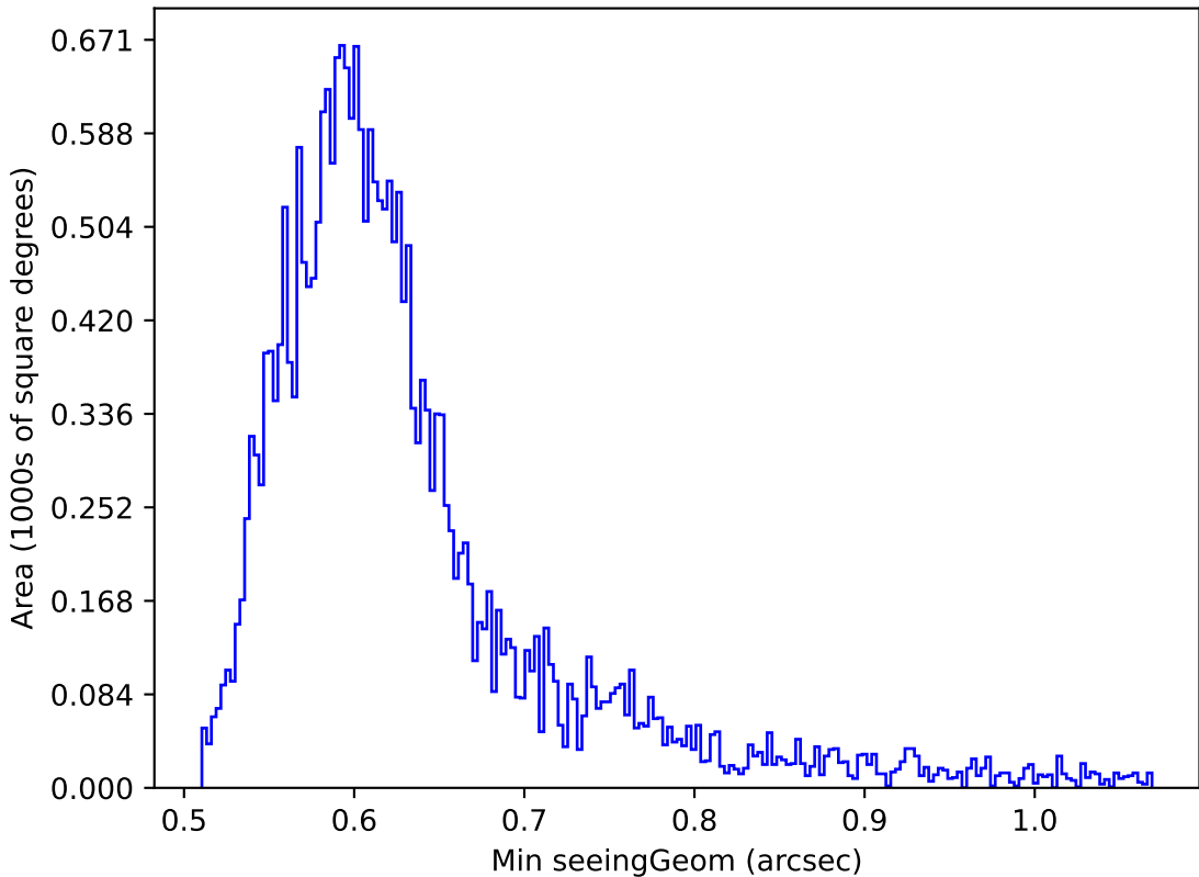
ddf_acor_sf30_lsf40_lsr20_v3.4_10yrs Yr 1 i band: Min seeingGeom
