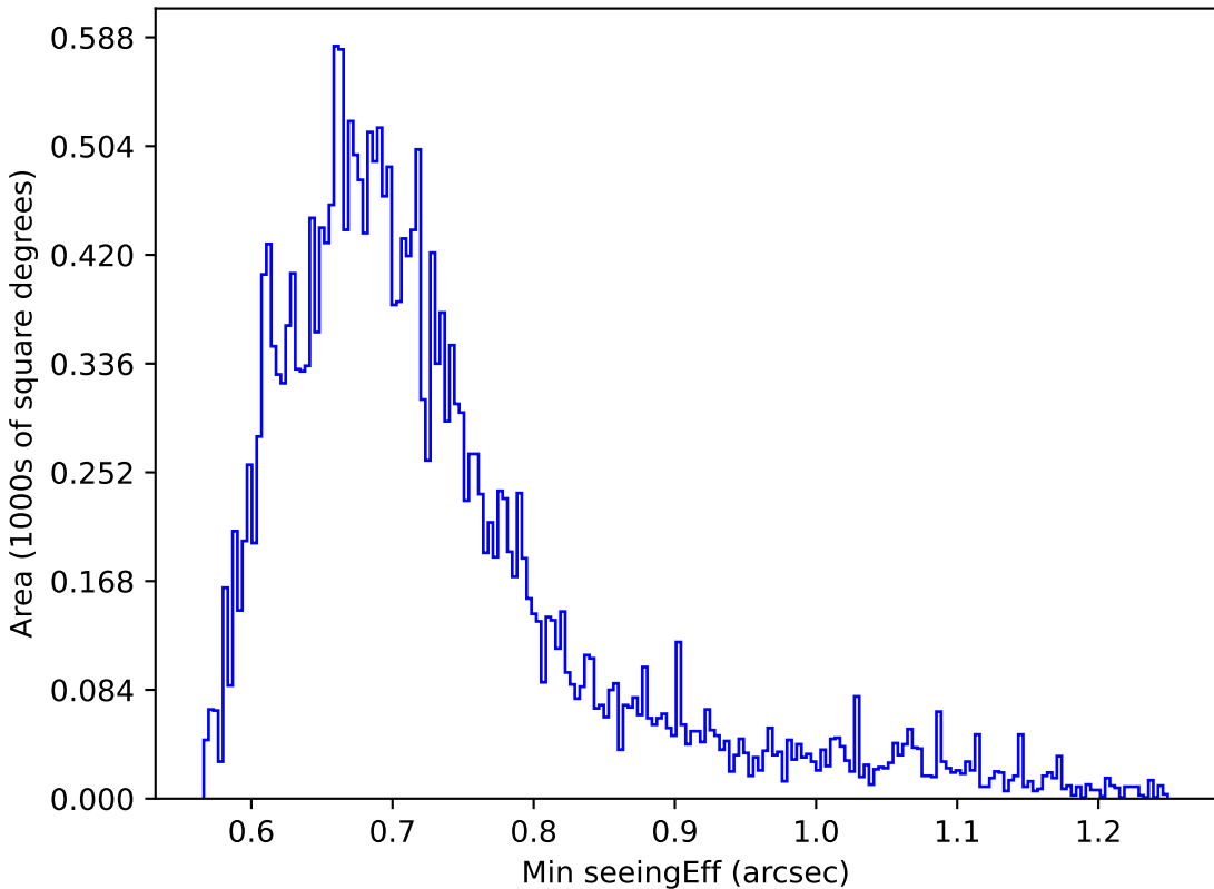
ddf_acor_sf30_ls40_lsr20_v3.4_10yrs Yr 1 z band: Min seeingEff
