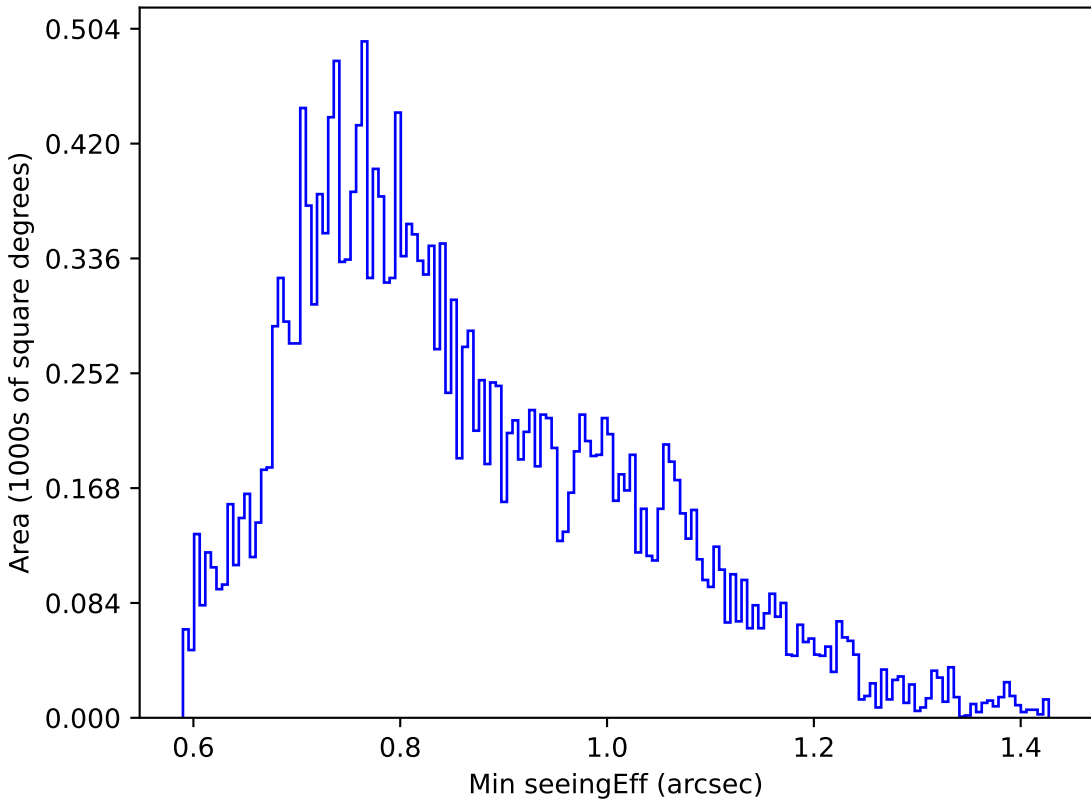
ddf_acor_sf30_lsf40_lsr20_v3.4_10yrs Yr 1 u band: Min seeingEff
