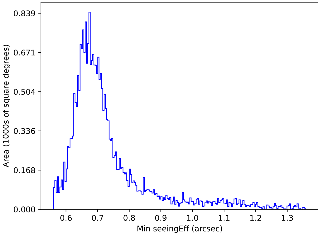
ddf_acor_sf30_lsf40_lsr20_v3.4_10yrs Yr 1 r band: Min seeingEff
