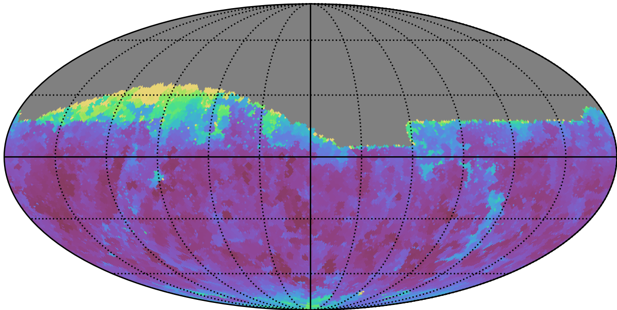
ddf_acor_sf30_lsf40_lsr20_v3.4_10yrs Yr 1 i band: Min seeingEff
