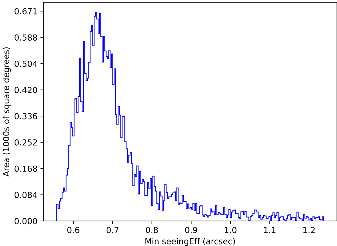
ddf_acor_sf30_lsf40_lsr20_v3.4_10yrs Yr 1 i band: Min seeingEff
