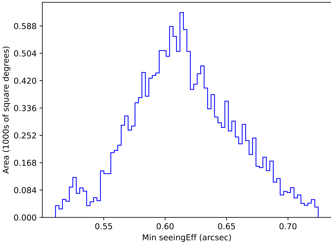
ddf_acor_sf30_lsf40_lsr20_v3.4_10yrs WFD z band: Min seeingEff
