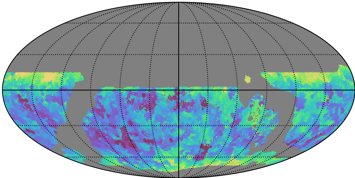
ddf_acor_sf30_lsf40_lsr20_v3.4_10yrs WFD y band: Min seeingEff
